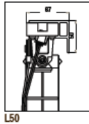
Head rail side view Detalle perfil cabezal
